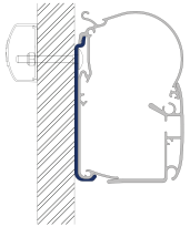
FLAT BRACKET
